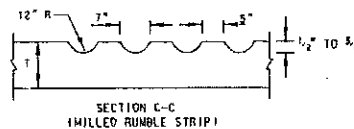
MILLED RUMBLE STRIP FOR PORTLAND CEMENT AND HOT MIX ASPHALT SHOULDERS
